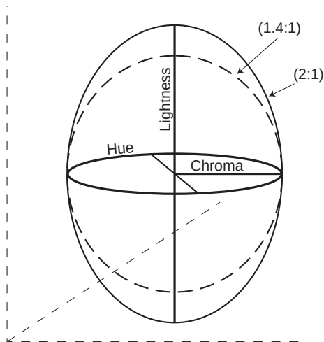
Figure 20: CMC tolerance ellipsoids
