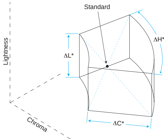
Figure 16: CIELCH tolerance wedge
