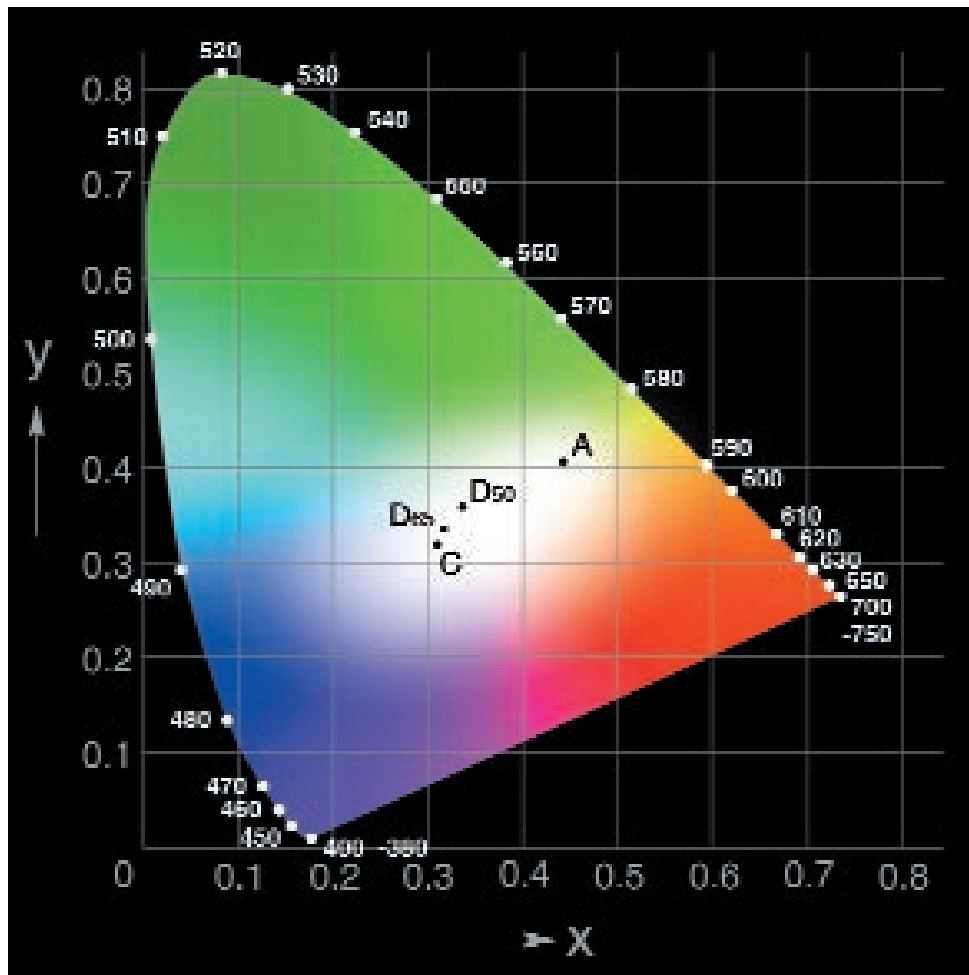
Figure 9: CIE 1931 (x, y) chromaticity diagram
