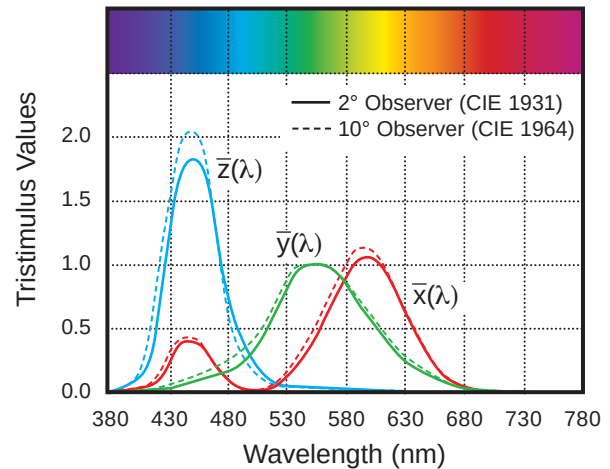
Figure 7: CIE 2° and 10° Standard Observers
