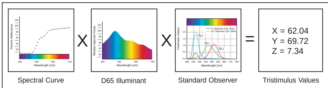
Figure 8: Tristimulus values
