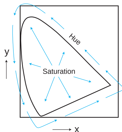
Figure 10: Chromaticity diagram
