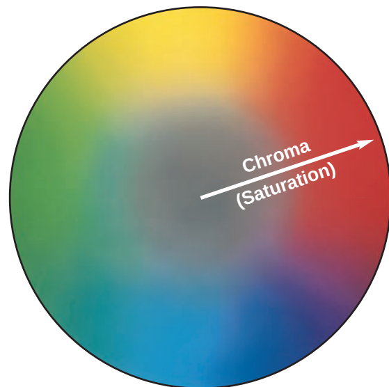
Figure 2: Chromaticity
