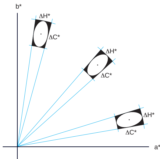
Figure 17: CIELCH tolerance ellipsoids
